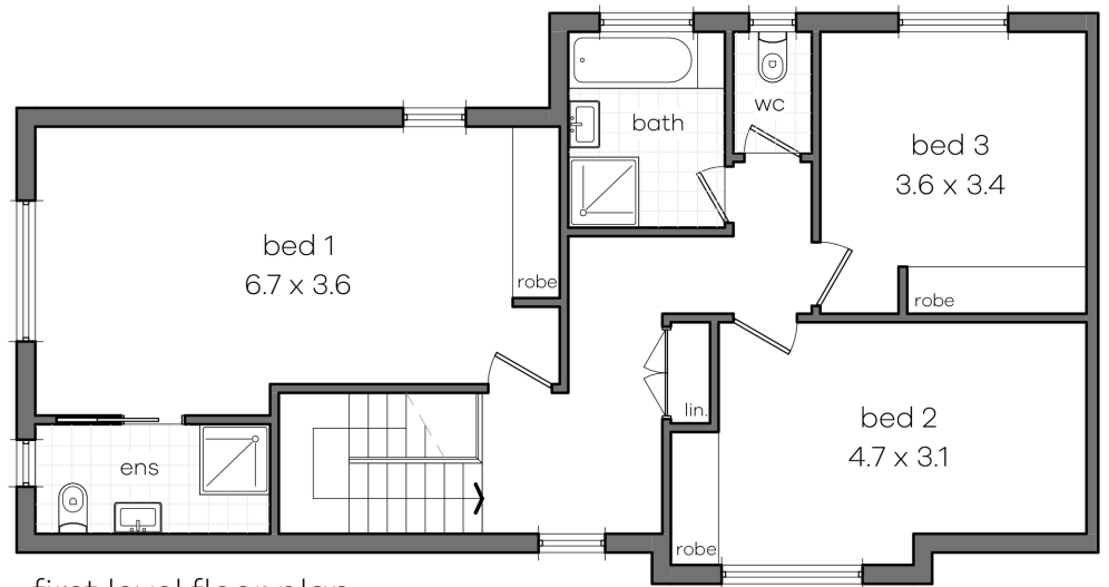
first level floor plan
