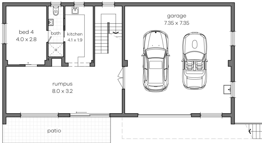
lower ground level floor plan
